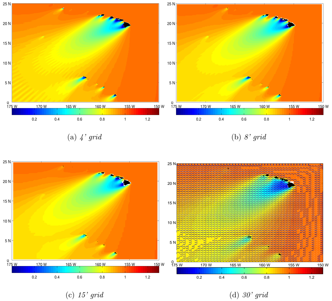
Fig. 3.13 : Normalized Significant wave heights for Test OB-2
