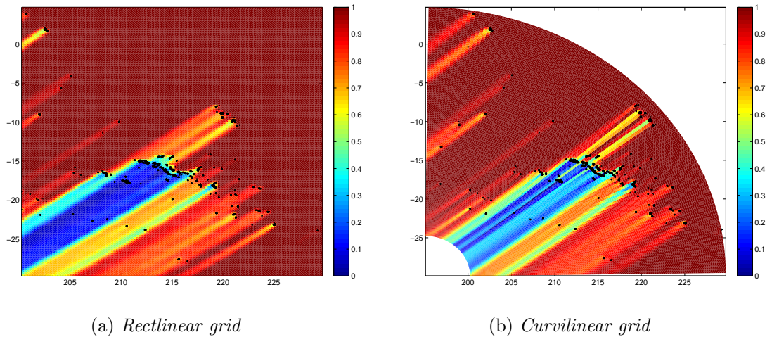
Fig. 3.27 : Swell propagation using a 1/4 deg rectilinear grid and a quarter annulus curvilinear grid. In both grids obstructions were generated considering neighboring cell information at both ends
