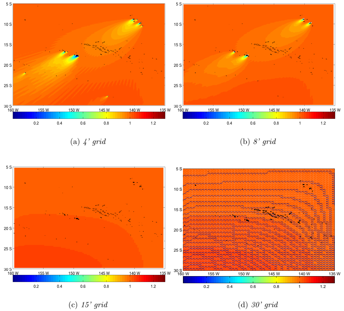
Fig. 3.21 : Normalized Significant wave heights for Test NO-OB
