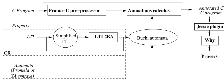
Figure 5.2: Plug-in Structure
